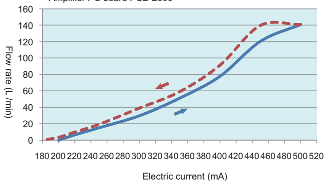
PV80 + Proportional flow valve PEV-16A-2D-09-N-1600 + Amplifier PC board PCB-2600
