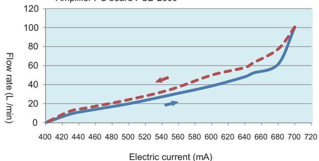
PV56+Proportional flow valve PFC-17E-2G-0700-N + Amplifier PC board PCB-2600
