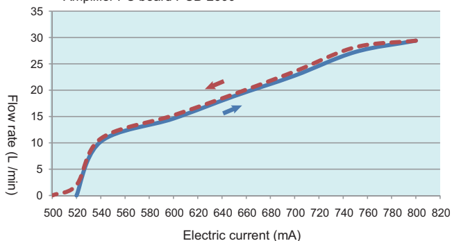
PV16 + Proportional flow valve PFC-17E-2G-0350-N + Amplifier PC board PCB-2600
