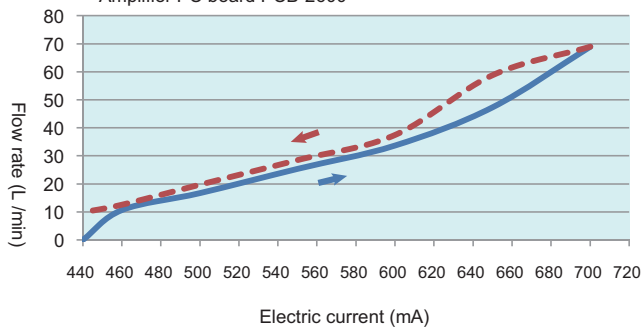
PV40 + Proportional flow valve PFC-17E-2G-0700-N + Amplifier PC board PCB-2600
