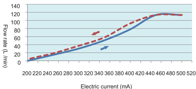
PV63 +Proportional flow valve PFC-17E-2G-0700-N + Amplifier PC board PCB-2600
