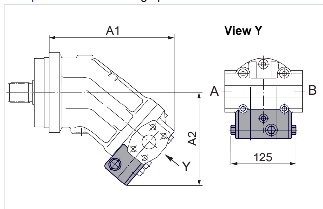
Port plate 029 – SAE flange ports at side
