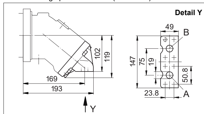
10 – SAE flange ports at bottom (same side)
