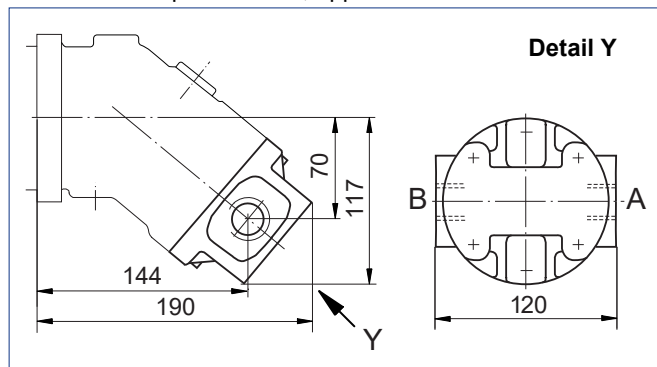
03 – Threaded ports at side, opposite
