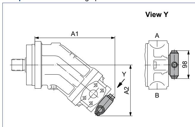
Port plate 027 – SAE flange ports at side
