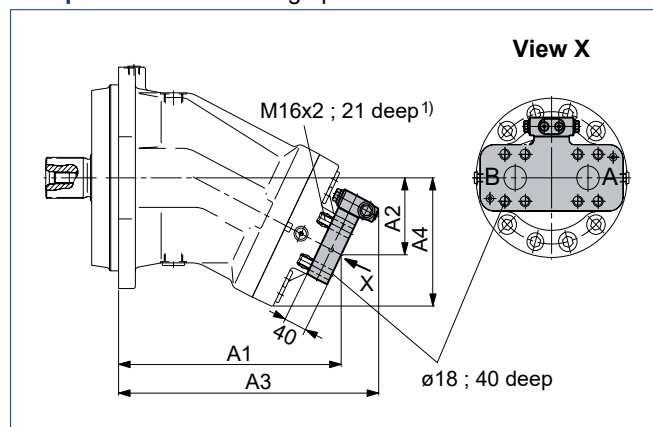
Port plate 017 – SAE flange ports at rear
