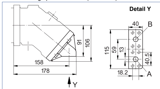
10 – SAE flange ports at bottom (same side) 4)
